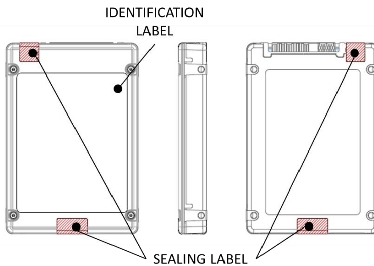
Exhibit 2 – Specification of the Samsung SAS 12G TCG Enterprise SSC SEDs PM1643 Series Cryptographic Boundary (From top to bottom, side).
