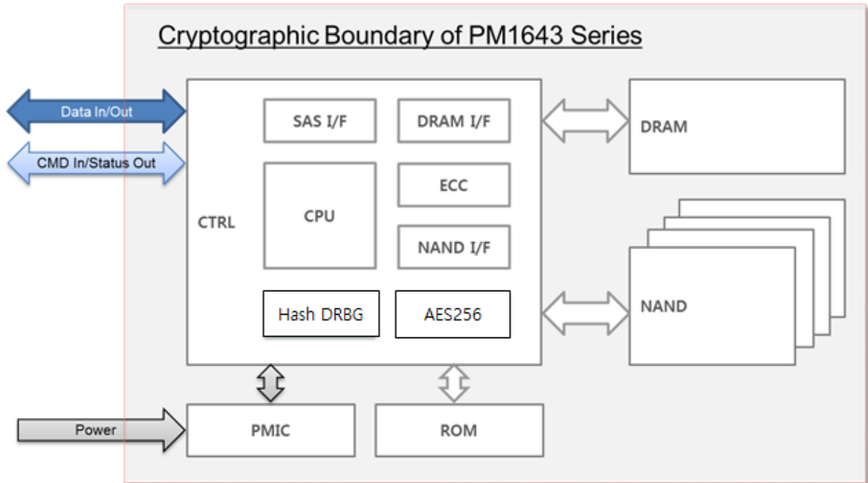
Exhibit 3 – Block Diagram for Samsung SAS 12G TCG Enterprise SSC SEDs PM1643 Series..
