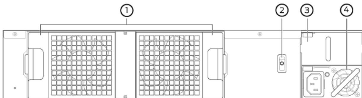
Figure 2- JA2500 Hardware Appliance Rear Panel
