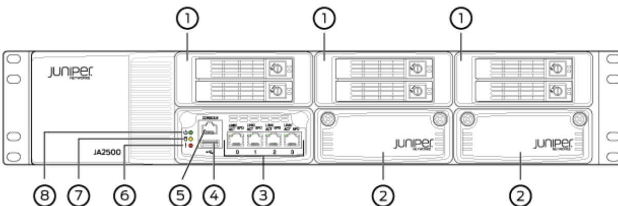
Figure 1- JA2500 Hardware Appliance Front Panel
