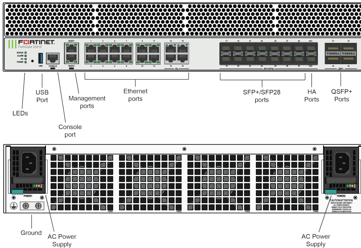
Figure 5 - FortiGate-3301E Front and Rear Panels
