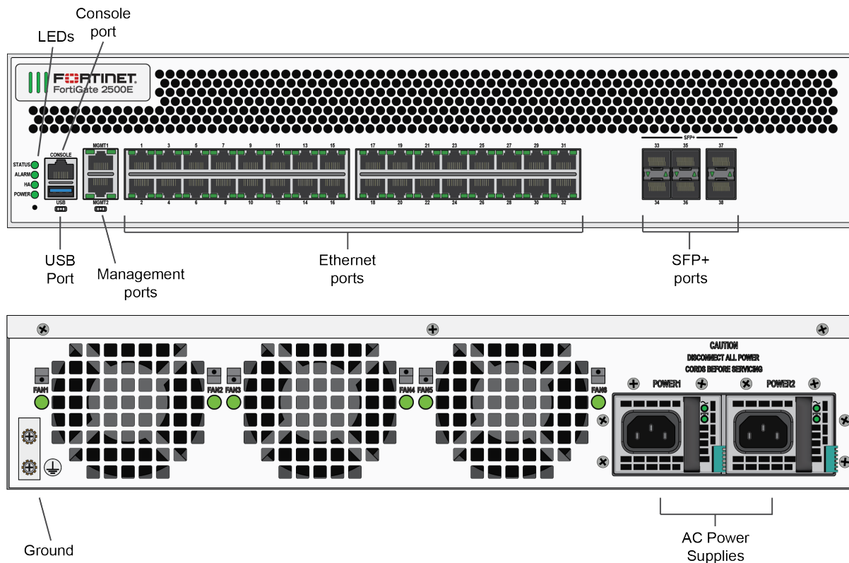
Figure 4 - FortiGate-2500E Front and Rear Panels
