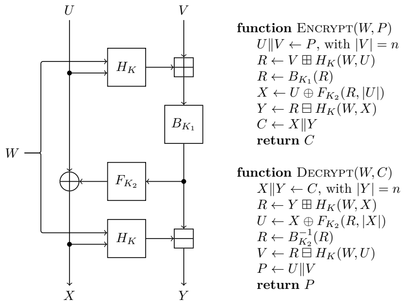
Figure 4: Adiantum mode (originally called HBSH in [CB18]).
