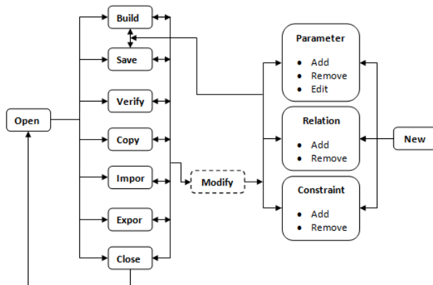
Figure 5: ACTS's Navigation Graph
