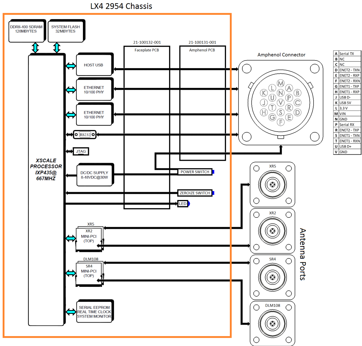
Figure 3: LX4-2954 Cryptographic Module Block Diagram
