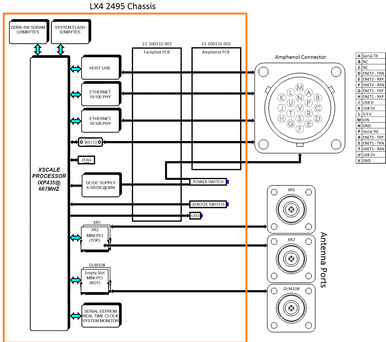
Figure 2: LX4-2495 Cryptographic Module Block Diagram
