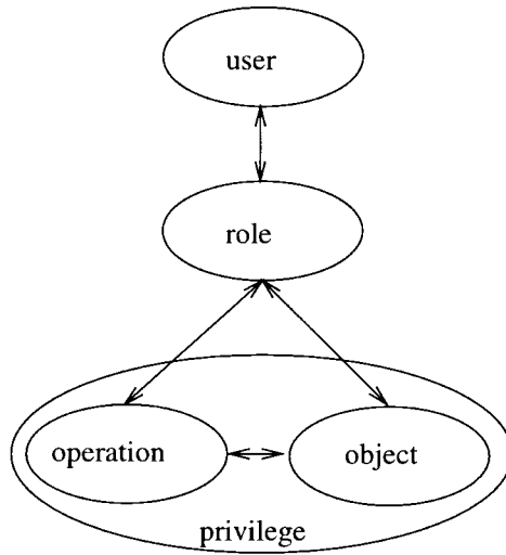
Fig. 1. Role-operation-object relationship.
