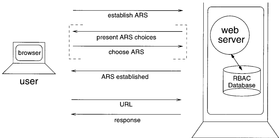
Fig. 8. RBAC/Web end-user perspective.
