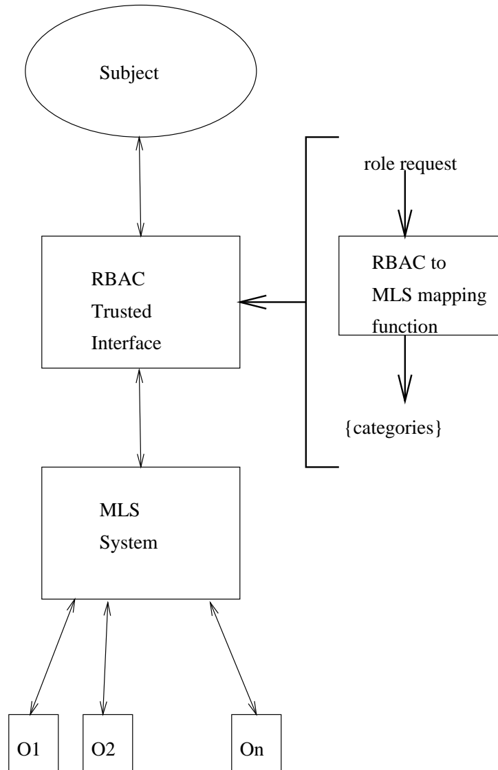
Figure 1: RBAC/MLS Interface
