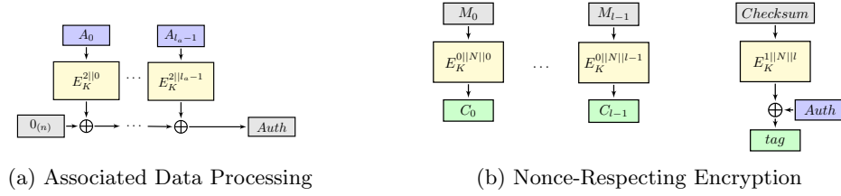
Fig. 3: Lilliput-AE's Nonce-Respecting Mode of Operation (without Padding)
