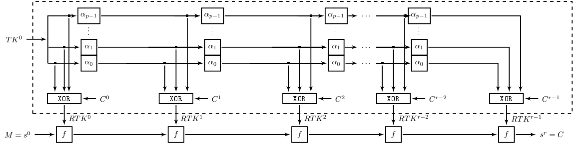
Fig. 2: Lilliput-TBC Tweakey Schedule
