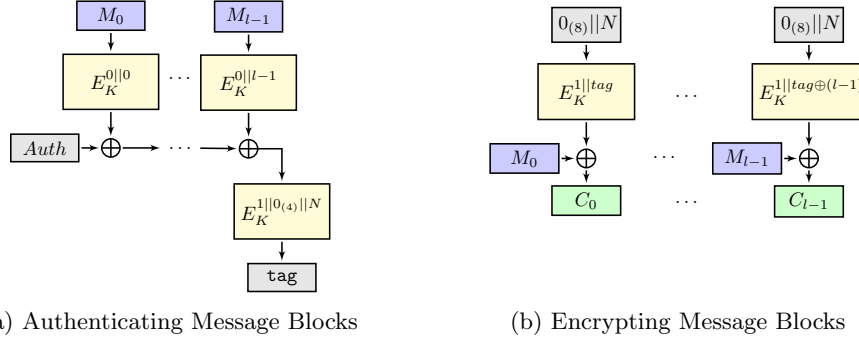
Fig. 4: Lilliput-AE’s Nonce-Misuse Resistant Mode of Operation (without Padding)
