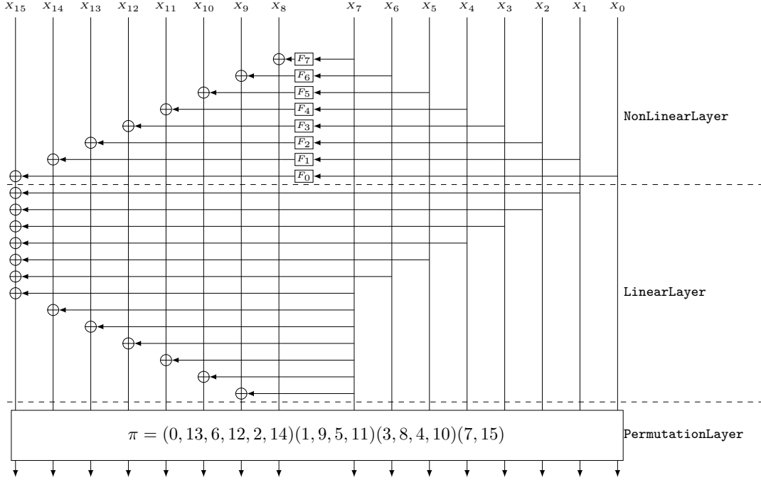
Fig. 1: Lilliput-TBC Round Function
