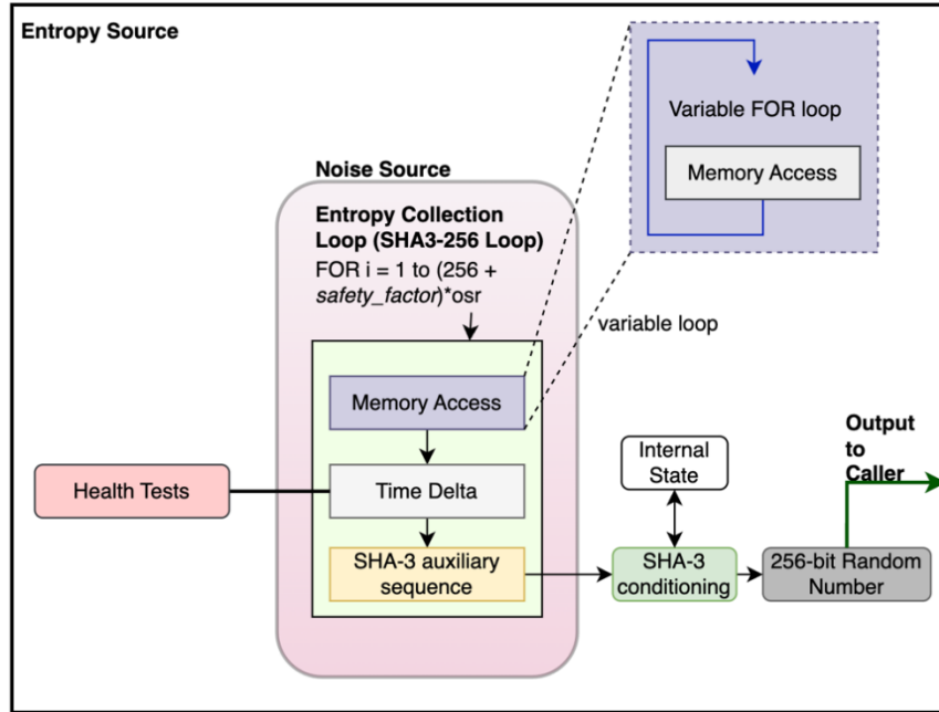
Figure 1: CPU Jitter 3.4.0 Design
