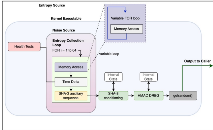
Figure 1: CPU Jitter 3.4.0 Design
