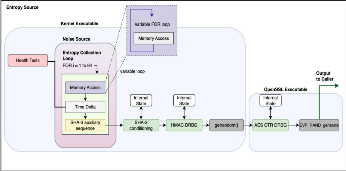
Figure 1: CPU Jitter 3.4.0 Design
