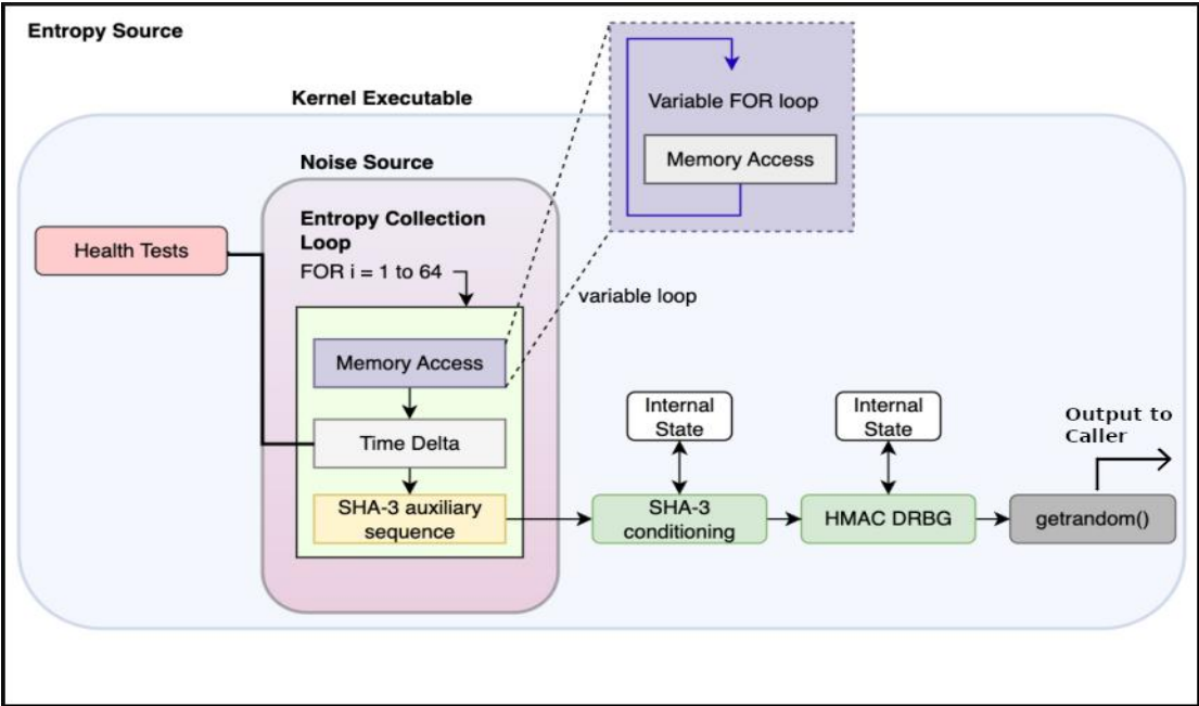
Figure 1: CPU Jitter 3.4.0 Design
