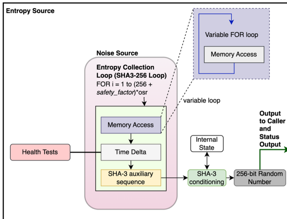
Figure 1: CPU Jitter 3.4.0 Design
