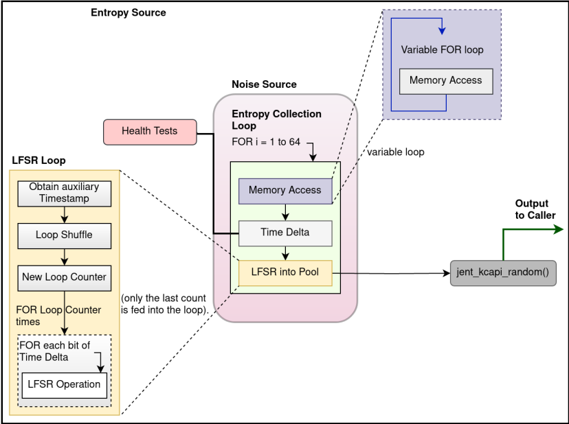
Figure 1: CPU Jitter 2.2.0 Design
