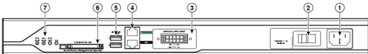
Figure 2 – 2811 Front Panel Physical Interfaces
