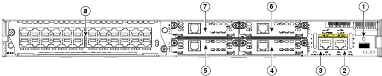
Figure 3 – 2811 Rear Panel Physical Interfaces
