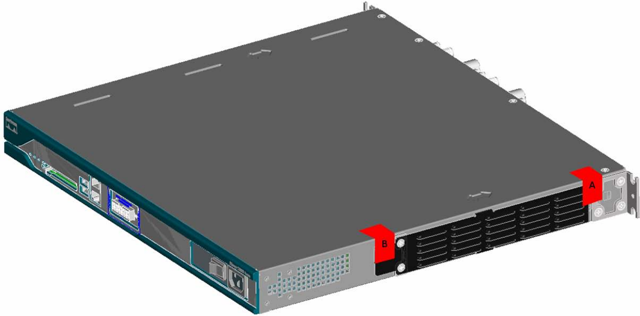
Figure 11 – 2811 Tamper Evident Label Placement on the Opacity Shield
