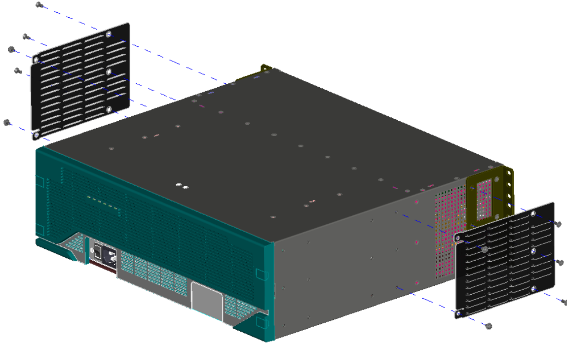
Figure 8 – 3845 – Opacity Shield Placement
