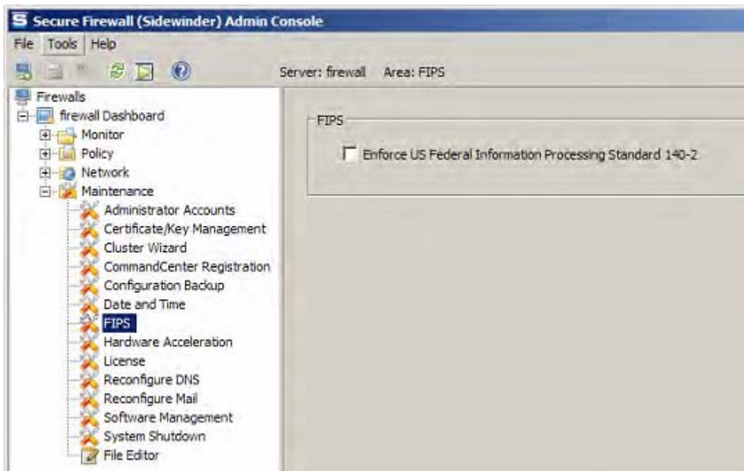
Figure 6 – Configuring For FIPS
