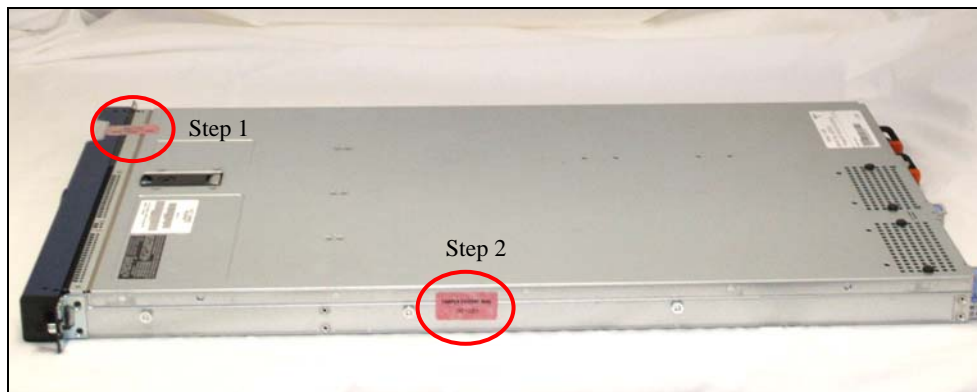
Figure 3 – Tamper-Evident Label Application Instruction for Secure Computing Secure Firewall (Sidewinder) 1100E
