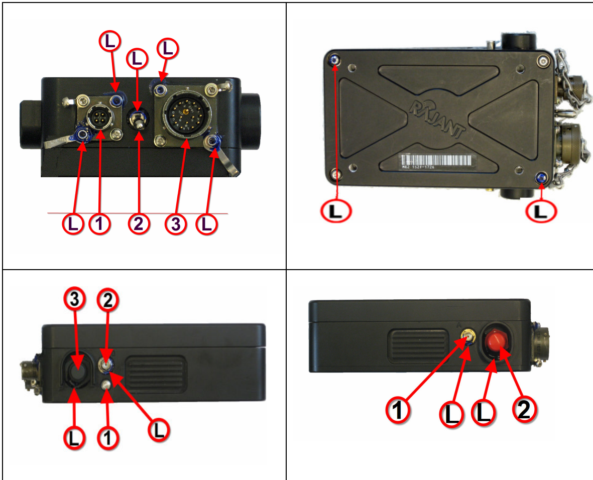
Fig 8.1 ME2 1S2F module views with 'loctite' compound over screws (blue color/ (L) label) for tamper evidence and resistance.
