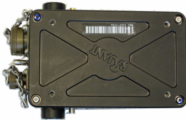
Figure 1.2: External view of the ME2 1S2F module.
