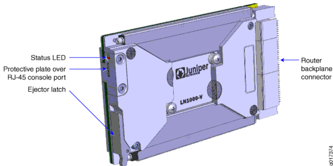
Figure 1: Depiction of the Cryptographic Module
