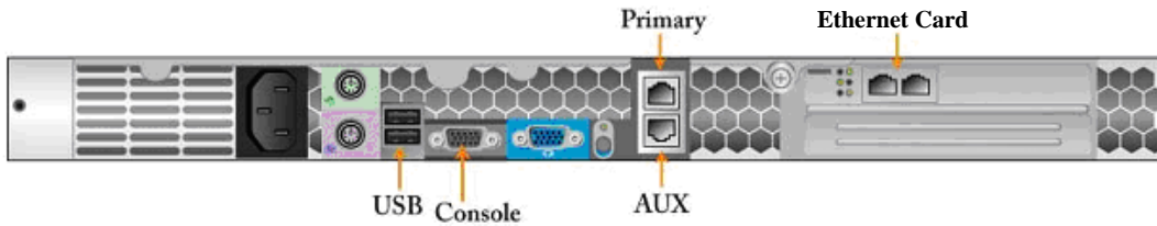
Figure 4 – Rear Panel of Steelhead 520, 1020, 1520, and 2020 Appliances
