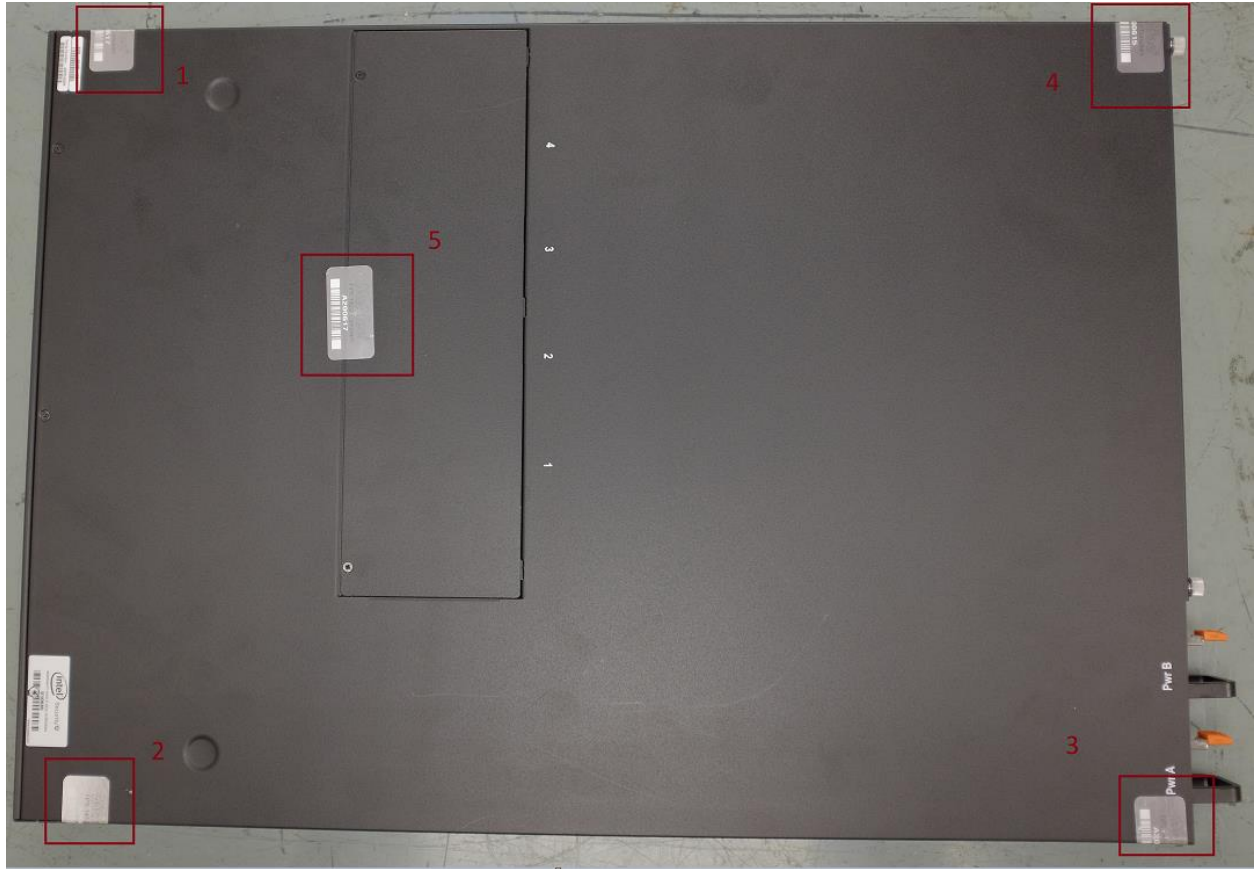
Figure 8 – Tamper Label Placement (NS5100/NS5200 Sensors)
