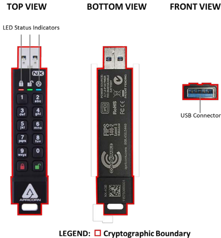
Figure 1 - Aegis Secure Key 3NX Cryptographic Module
