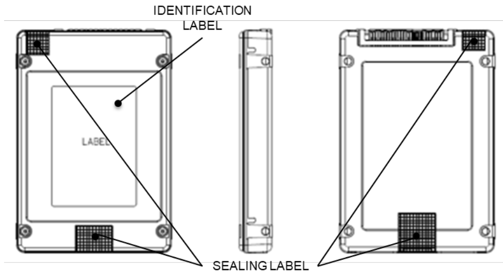
Exhibit 2 – Specification of the Samsung NVMe TCG Opal SSC SEDs PM1733 Series Cryptographic Boundary (From top to bottom, side).
