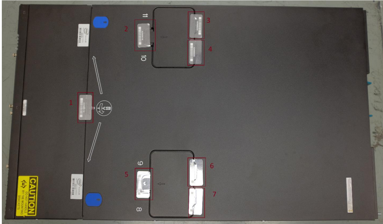
Figure 4 – Tamper Label Placement Top (NS9100/NS9200 Sensors)
