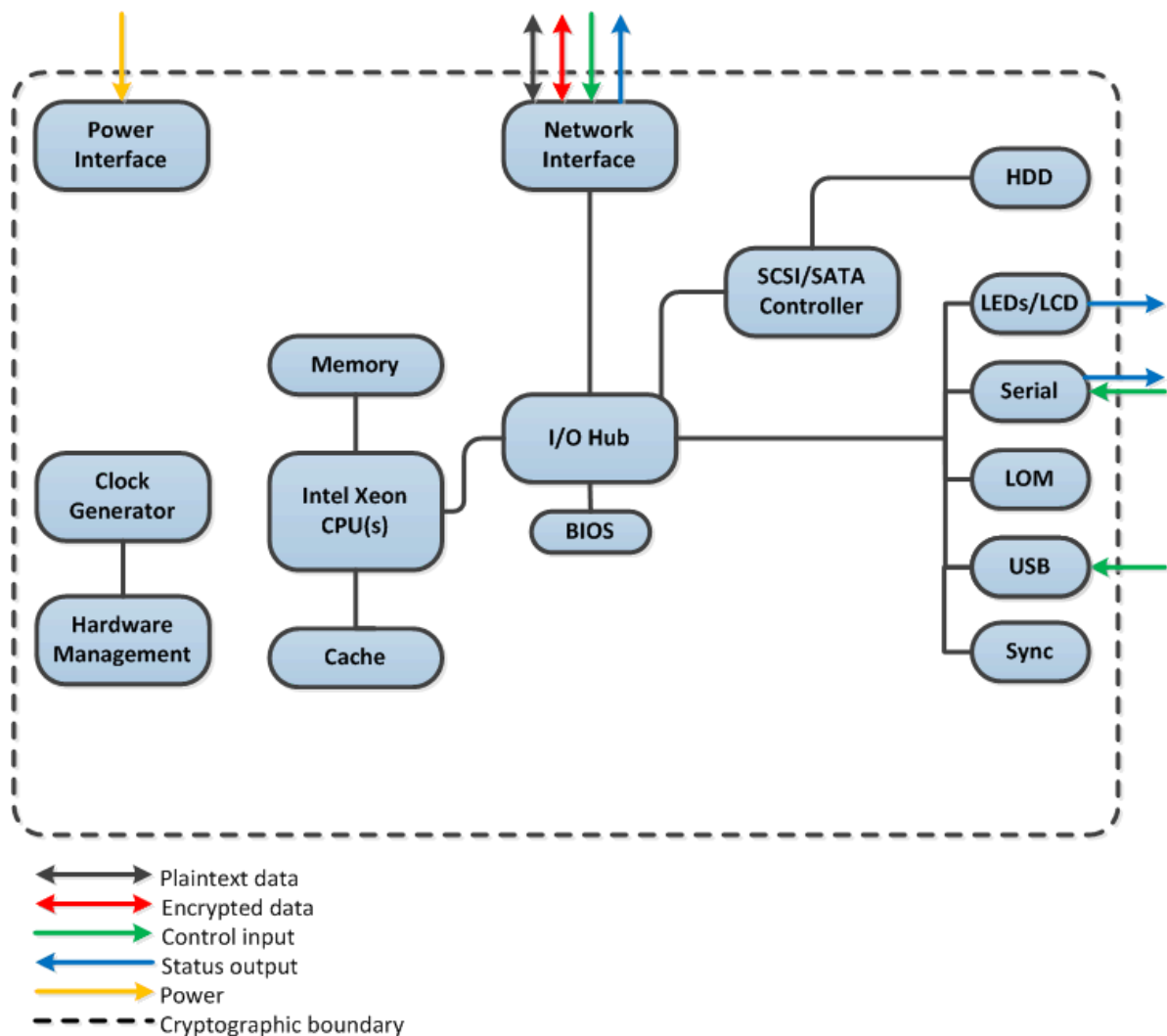
Figure 4 Block diagram for Check Point 1530/1535/1550/1555/1570/1575/1570R/1575R/1590/1595/1600/1800/3600/7000/16200 Plus/28000, 9100, 9300, 9400 appliance hardware and HPE DL360 gen 10
