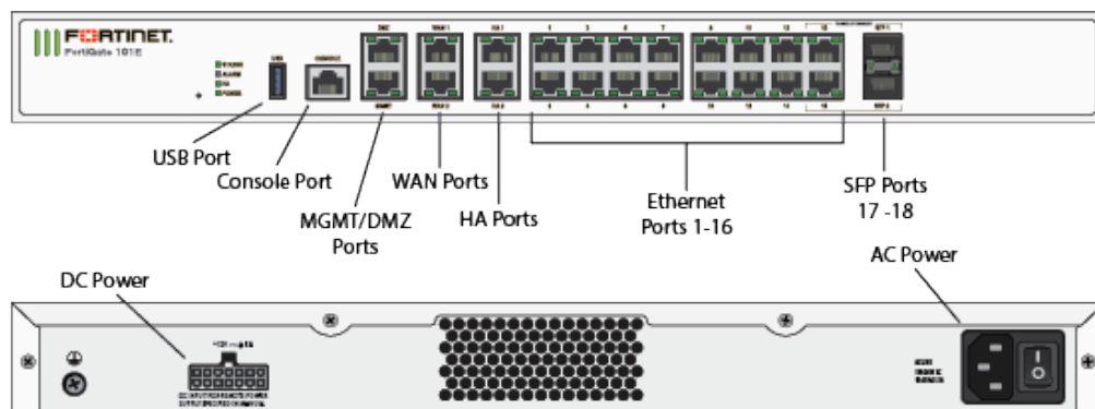
Figure 4 - FortiGate-101E Front and Rear Panels
