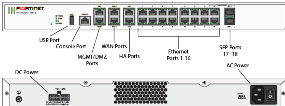
Figure 5 - FortiGate-101F Front and Rear Panels
