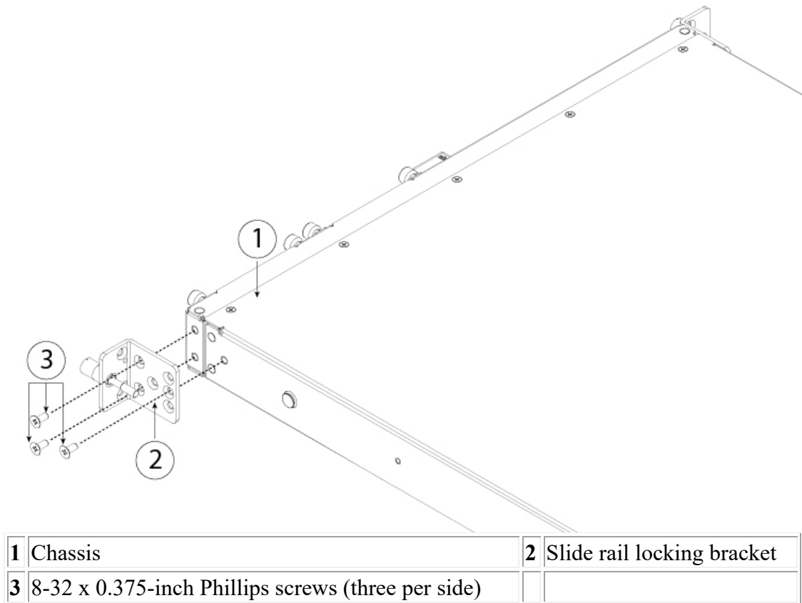
Figure 15. Attach the Slide Rail Locking Bracket to the Side of the Chassis
