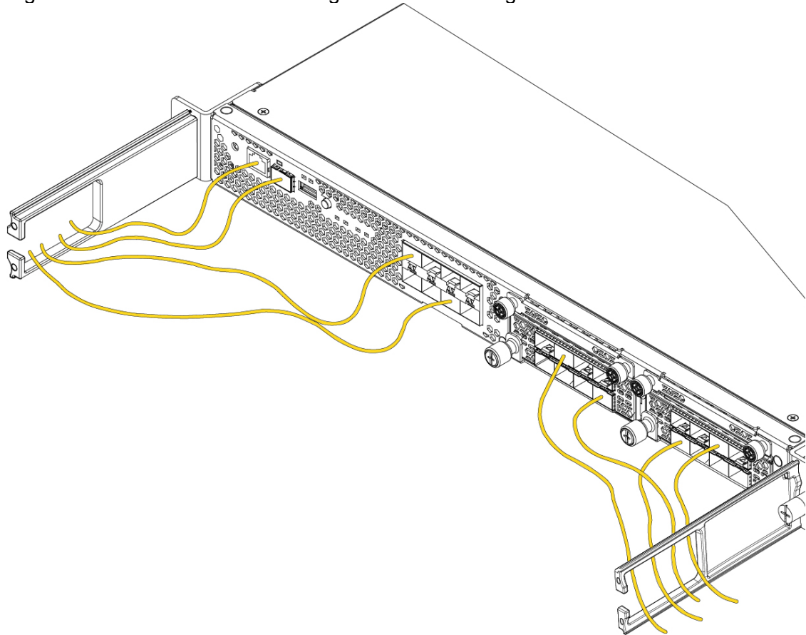
Figure 17. Route the Cables Through the Cable Management Brackets
