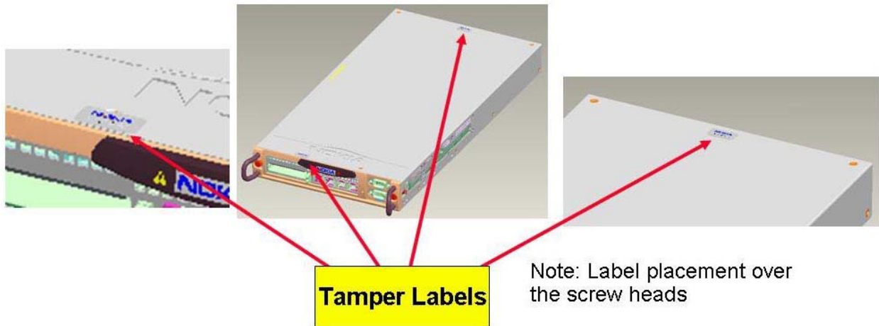
Figure 2 – Tamper Seal Location for a 1U Half-Width Chassis (2 Seals; covers access screws on top of unit)
