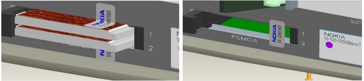
Figure 4 – Tamper Seal Location(s) for PCMCIA Flash Memory Bay (a 1U Half-Width Chassis with 2 Seals shown in left picture; a 2U Chassis with 1 Seal shown in right picture)
