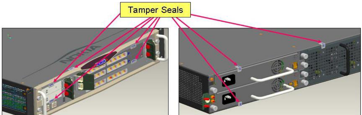
Figure 3 – Tamper Seal Locations for a 2U Chassis (8 Seals)
