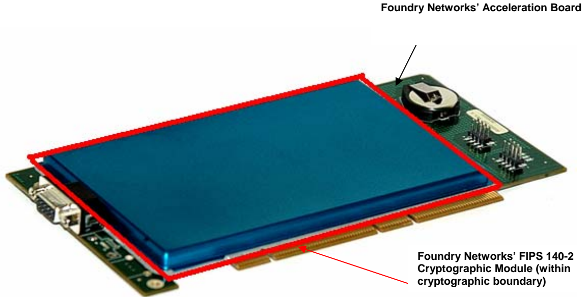
Figure 2-1. Foundry Networks' FIPS 140-2 Cryptographic Module, Level 3
