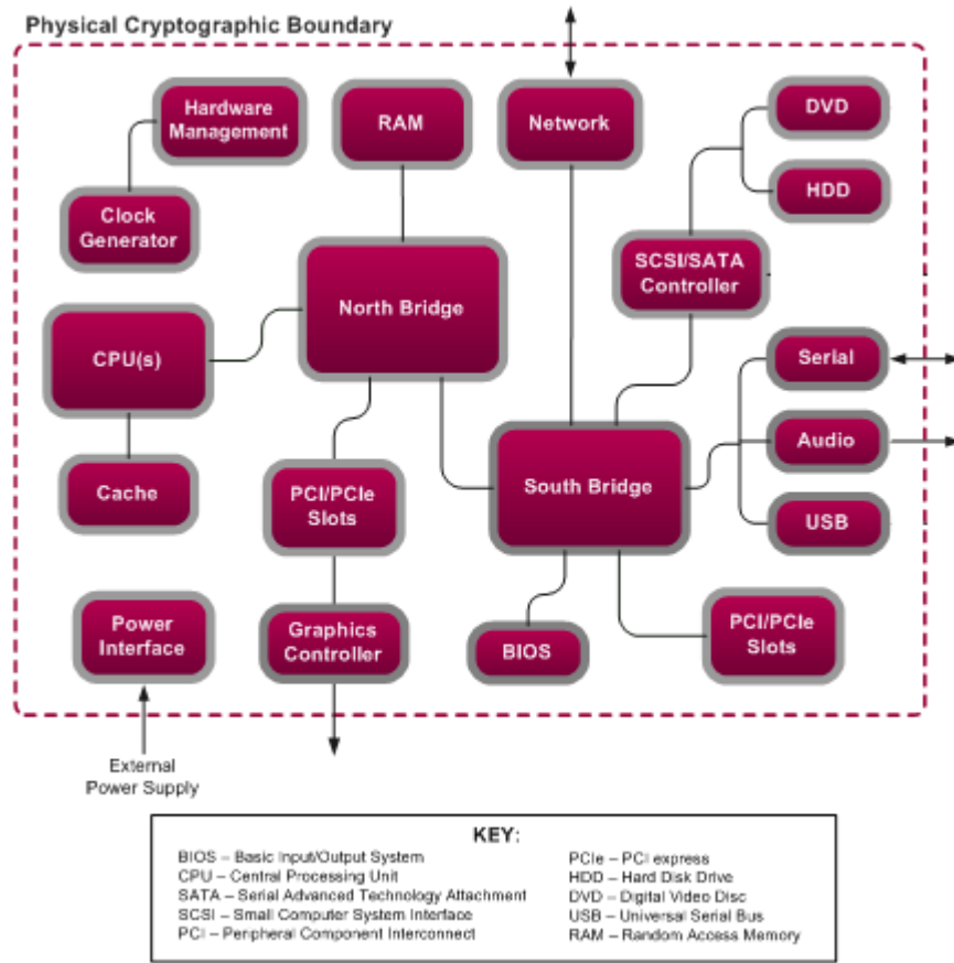
Figure 2 - GPC Block Diagram
