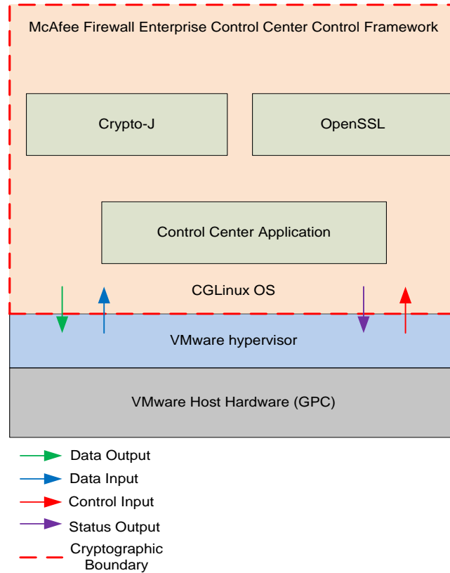
Figure 3 - Control Center Logical Cryptographic Boundary
