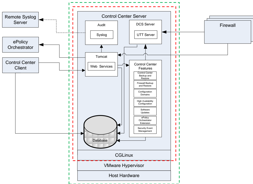
Figure 1 - Control Center Virtual Appliance Architecture
