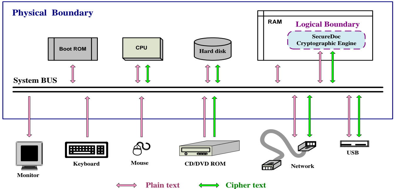
Figure 1 - Cryptographic Module Block-Diagram
