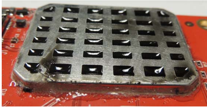
Figure 10 Cryptographic boundary (Top Picture)
