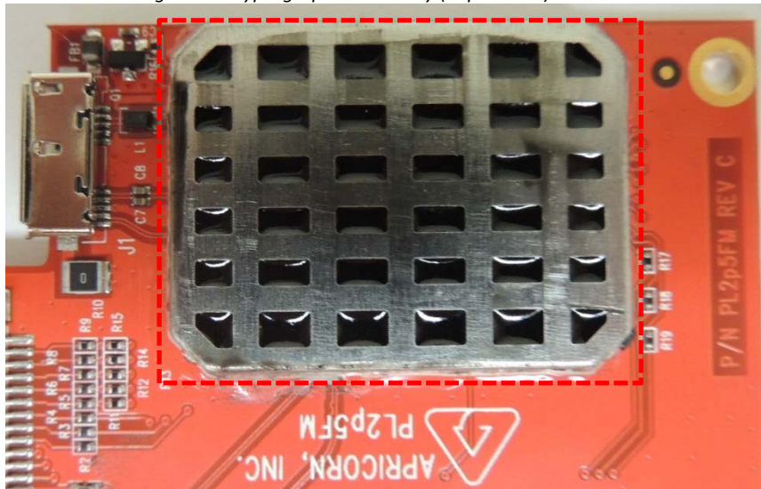
Figure 10 Cryptographic boundary (Top Picture)
