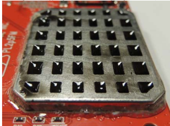
Figure 8 Cryptographic Boundary (Right Picture)
