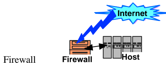
Replicated/Distributed System
