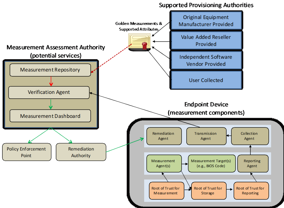
Figure 1: BIOS Integrity Architecture
